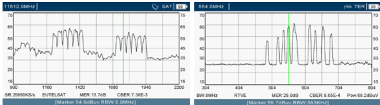
Satellite and terrestrial signals spectrum
