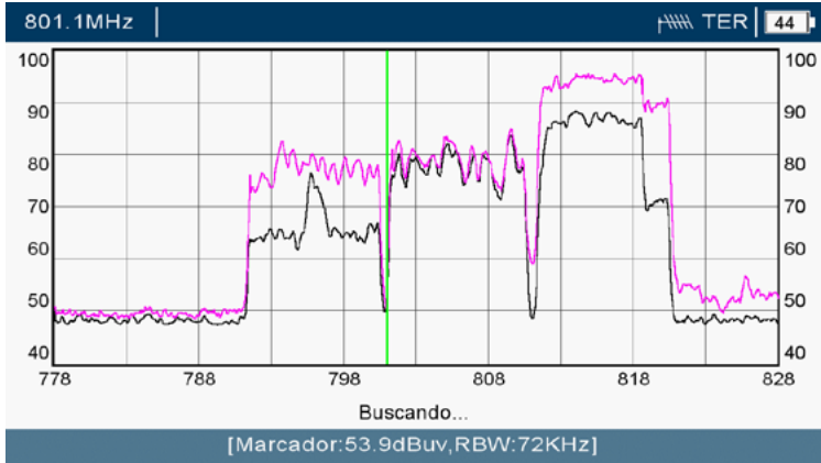
Measurement at the head of an interfering signal 4G. (The downlink channels are observed)
