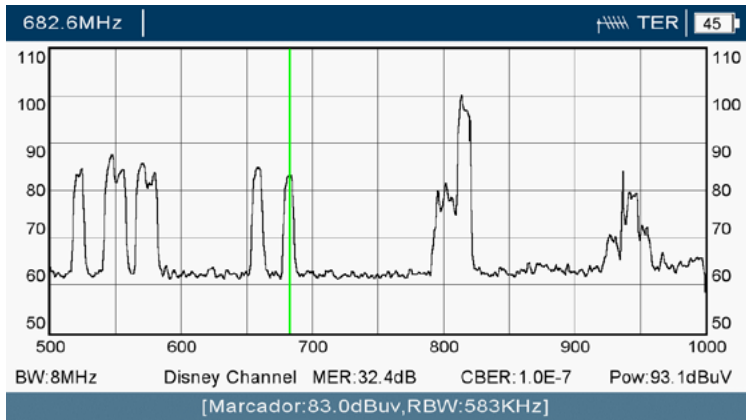
Measurement at the head including 3G and 4G signals (The downlink channels are observed at DVB-T channels)
