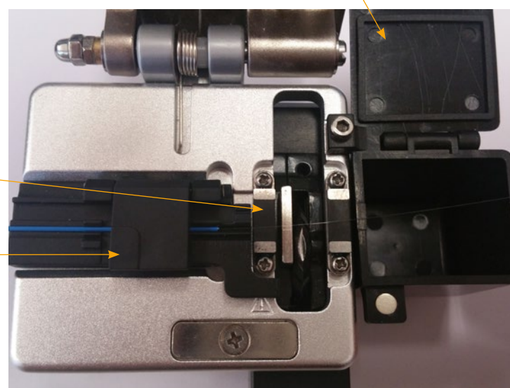
Cleaver detail with fibre optic ready for cutting
