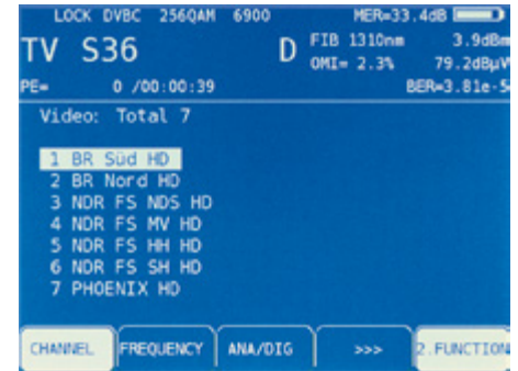
Measurement of an optical CATV signal with evaluation of all familiar RF parameters.
